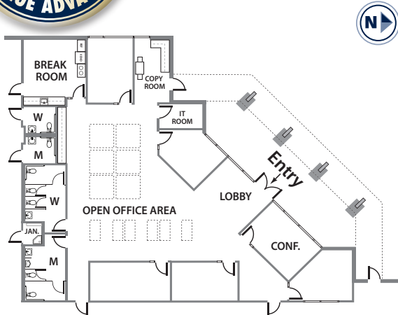
726.1 OFFICE PLAN 3,408 SF
