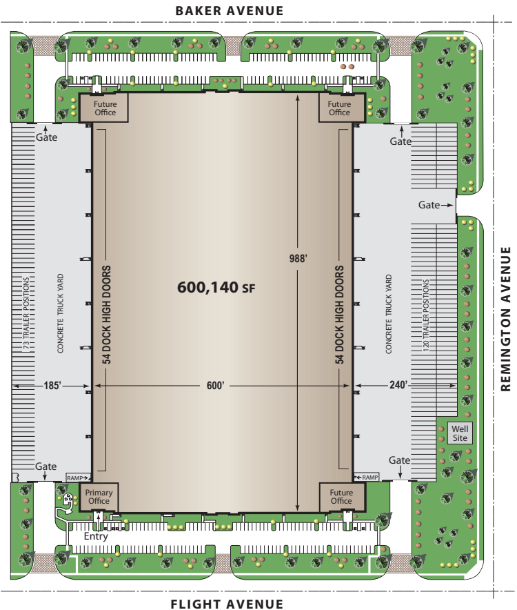
LEGACY BUILDING SM 837 SITE PLAN
