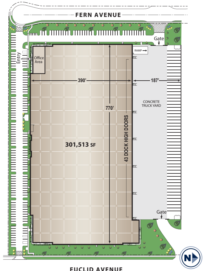
LEGACY BUILDING SM 819 SITE PLAN
